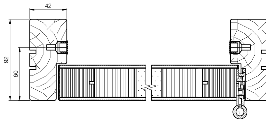
Unrebated WET ROOM ds (floor -30 mm) Installation
